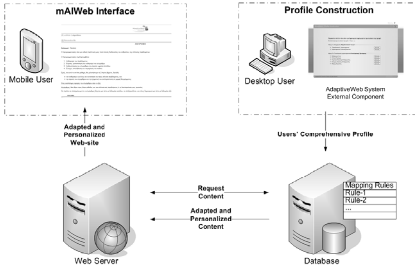
Figure 2. mAIWeb System Architecture
